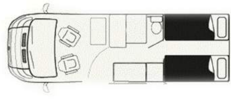
Vista 3 Twin Night 2
